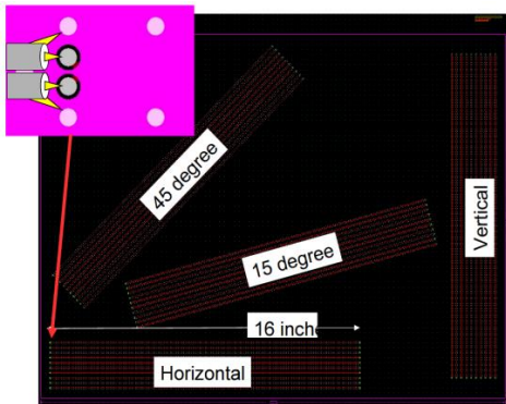
out of skew test vehicle for EZIO/EZIO Layout of skew test vehicle for EZ-IO/EZ-IO-F and fastRise™ prepreg.
