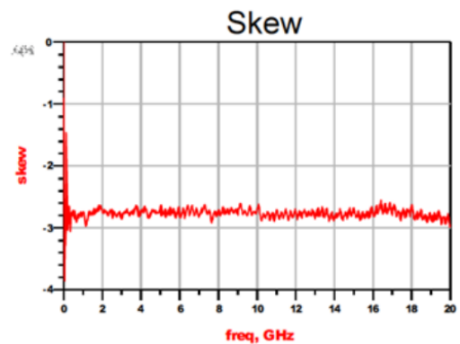
Skew testing of EZ-IO/EZ-IO-F and fastRise™ consistently showed the skew to be independent of frequency.
