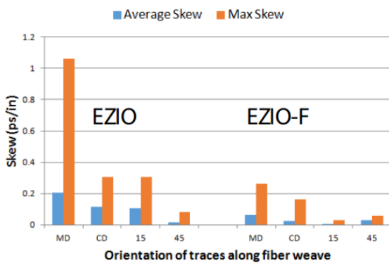
Average skew and maximum skew of paired transmission lines as a function of angle.
