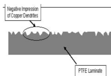
Figure 3 - Illustration of PTFE surface remaining after copper removal / etching
