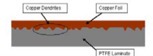
Figure 1 - Illustration of copper laminated to PTFE surface
