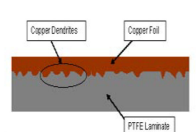
Figure 2 - Illustration of copper laminated to PTFE surface
