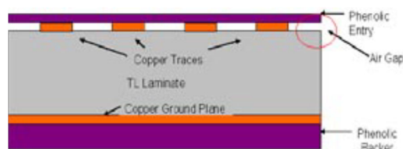
Figure 5 - A typical rout stack
